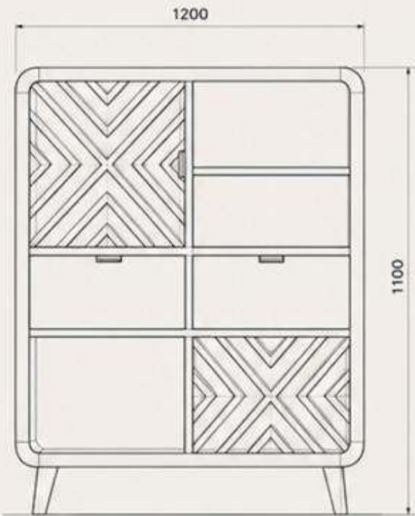
VISTA FRONTAL
