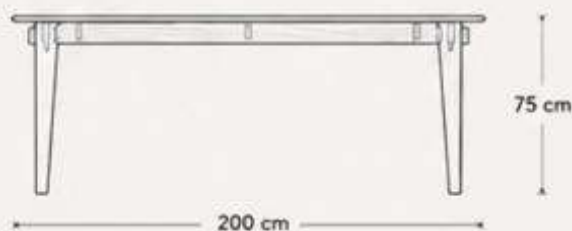
VISTA FRONTAL
